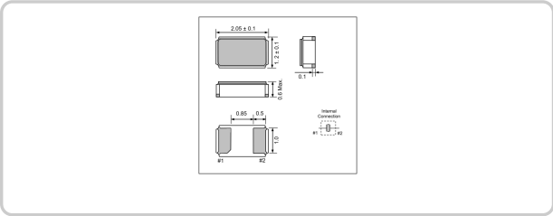
MARKING DIMENSION
